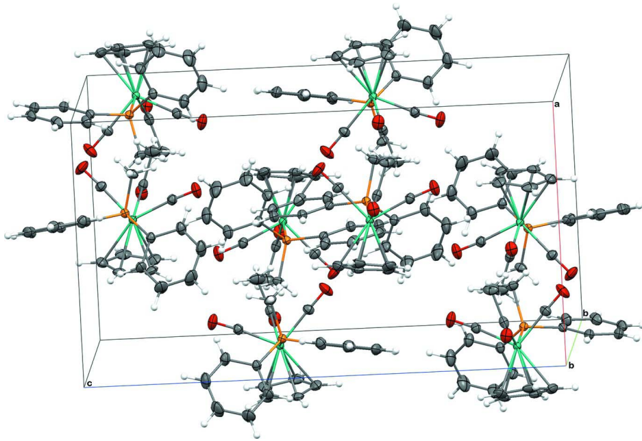
Figure 3 Unit cell packing diagram of (I) (50% probability ellipsoids).
