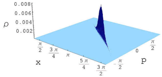
FIG. 7. (Color online) Previous state after evolution in the pendulum potential, at t=1.0 , when the distribution has contracted along the stable manifold.
