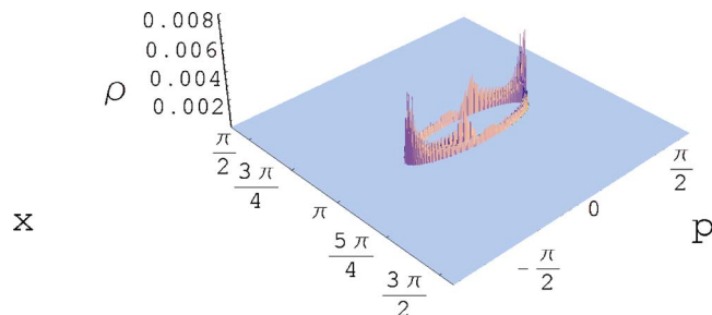
FIG. 15. (Color online) The distribution from Fig. 14 seen much later (at T=2400 kicks) showing that the dephasing has lead to an incoherent distribution spread across the accessible orbits.
