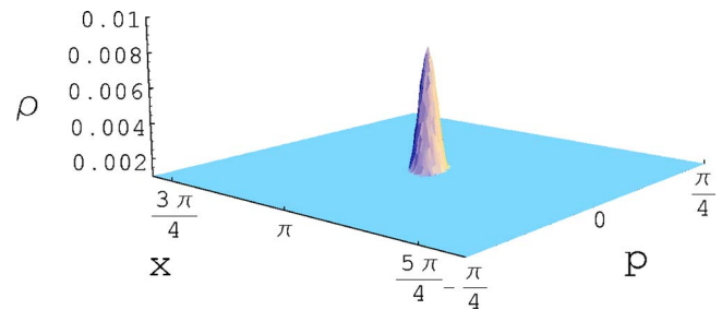
FIG. 8. (Color online) Same as above, at t=2.5 . Note the change of scale on all three axes. The distribution is now sharply focused at the unstable fixed point.
